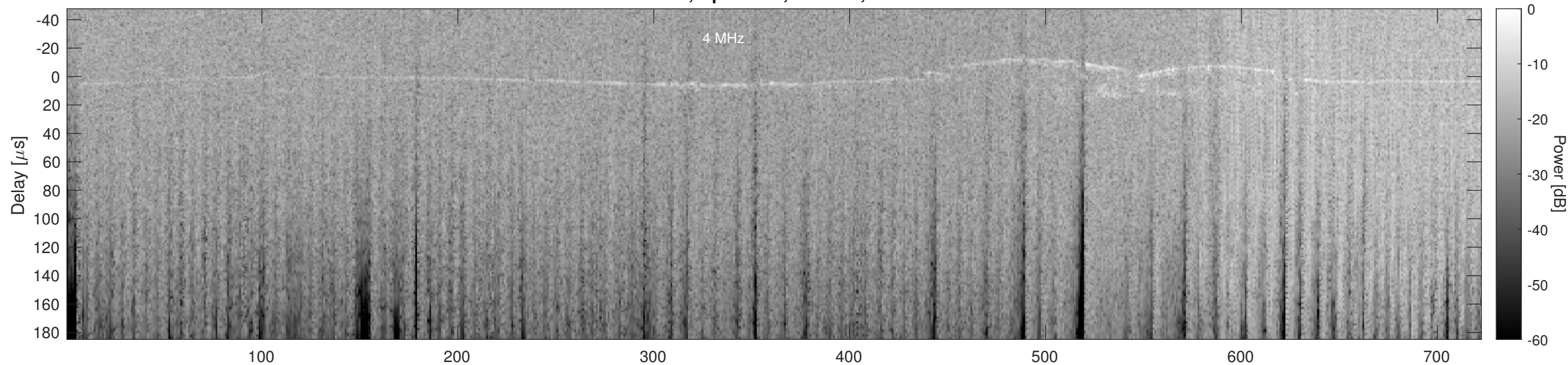
Orbit 13946, Optimized, Window, Channel 2
