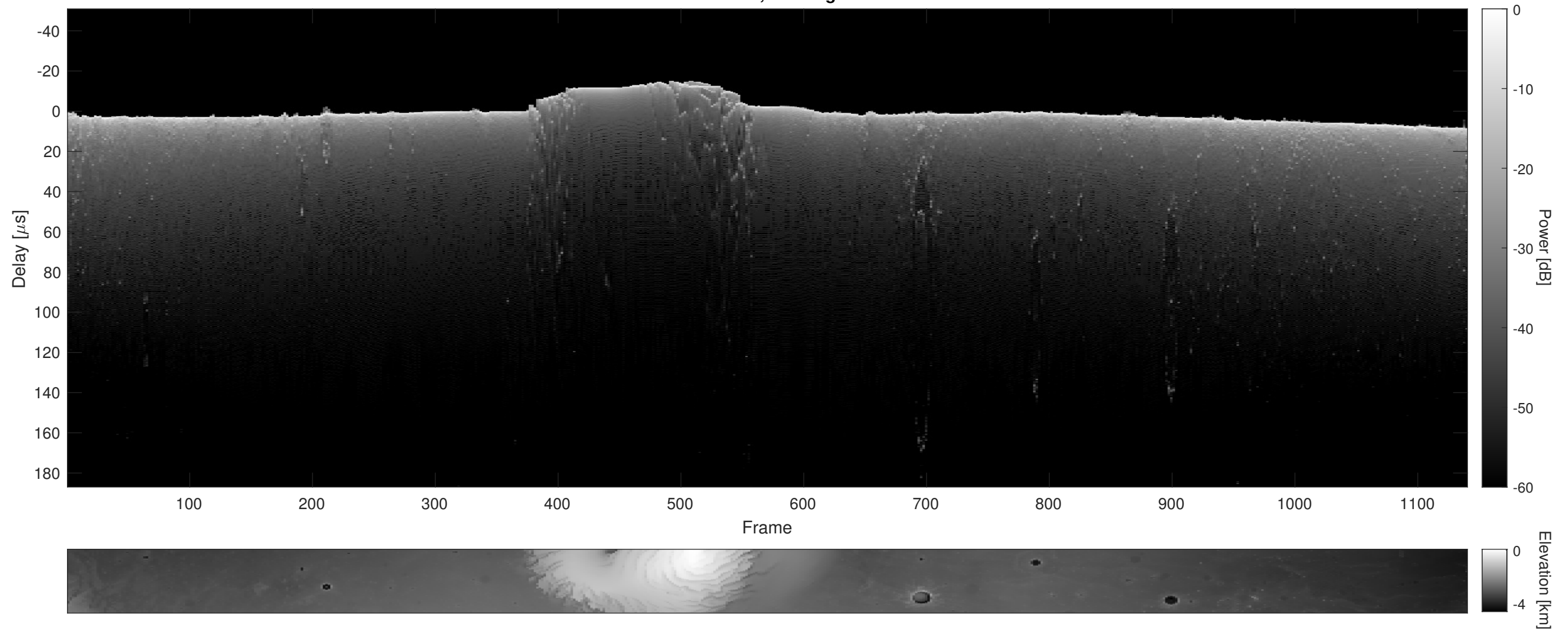
Orbit 13948, Cluttergram
