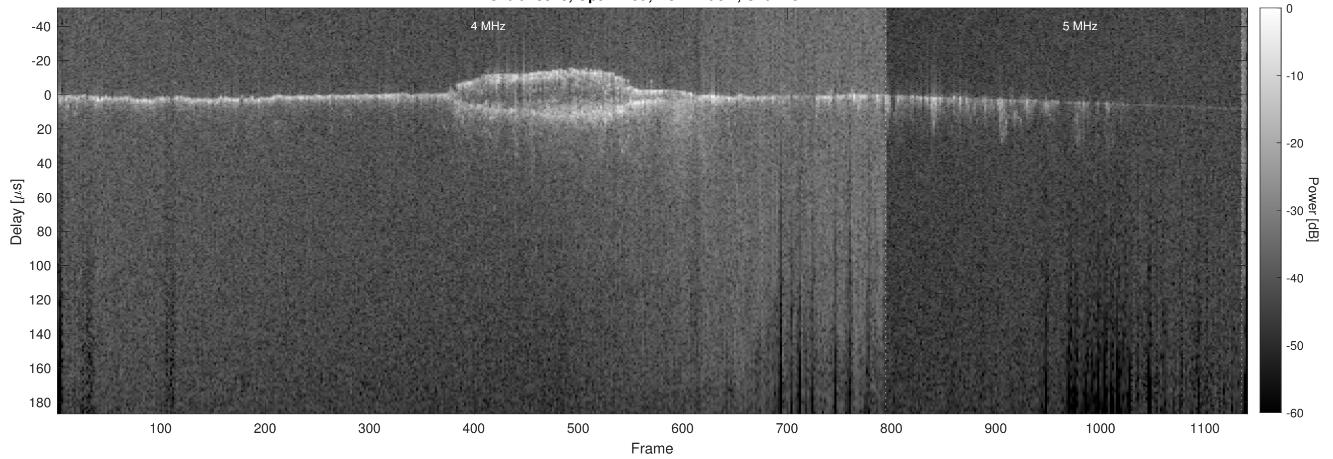
Orbit 13948, Optimized, No Window, Channel 2
