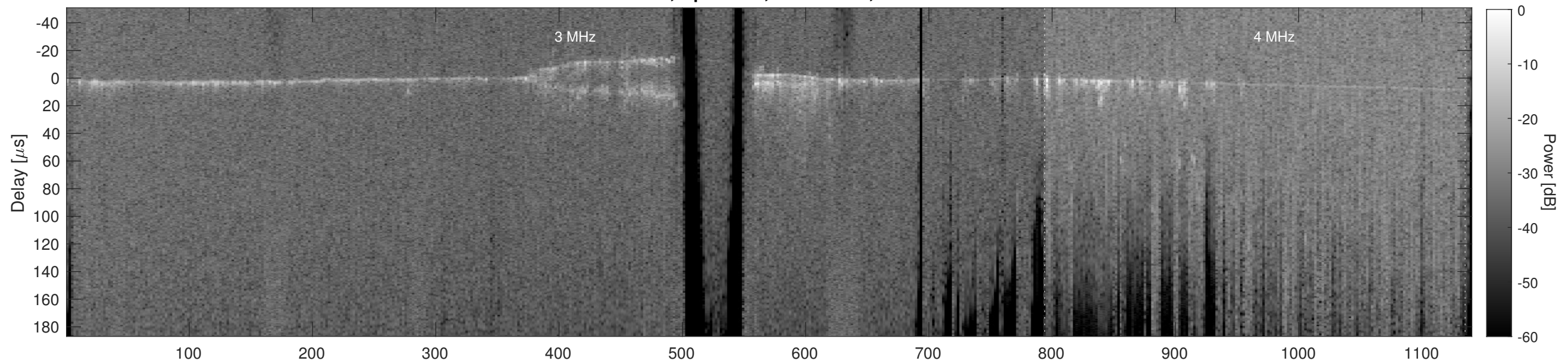
Orbit 13948, Cluttergram
