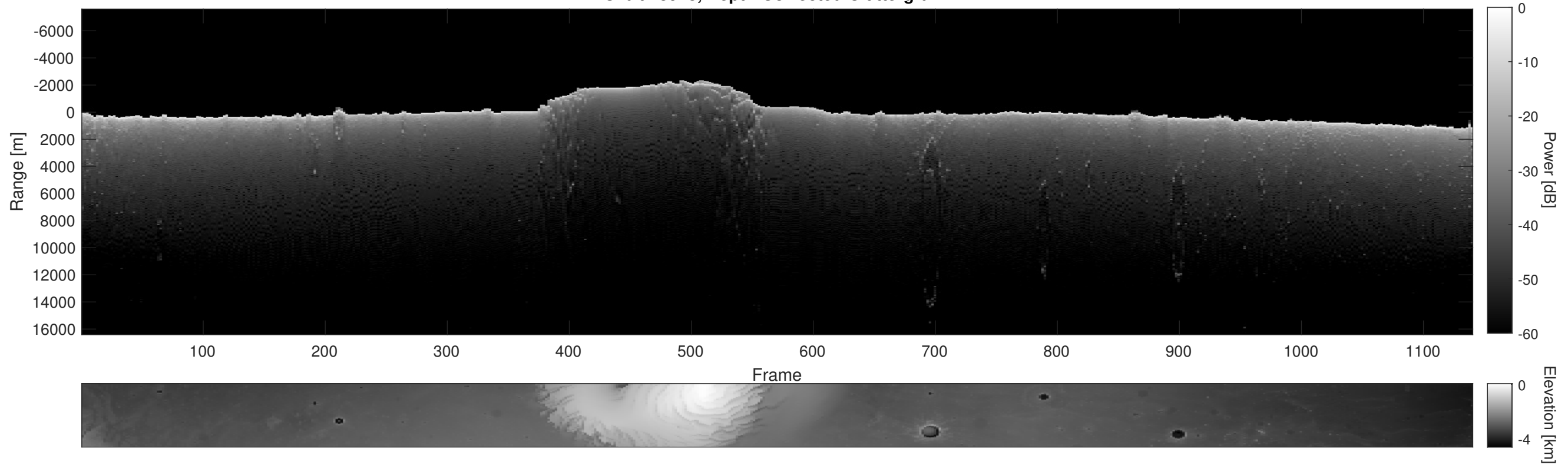
Orbit 13948, Depth-Corrected Cluttergram
