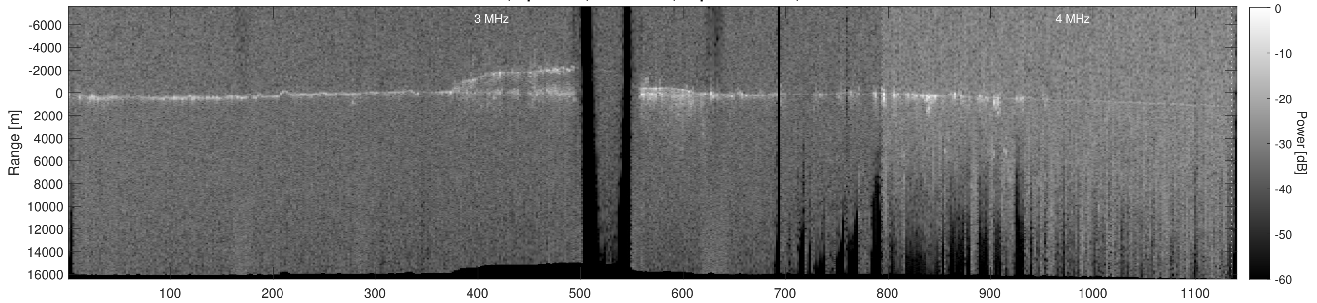
Orbit 13948, Depth-Corrected Cluttergram
