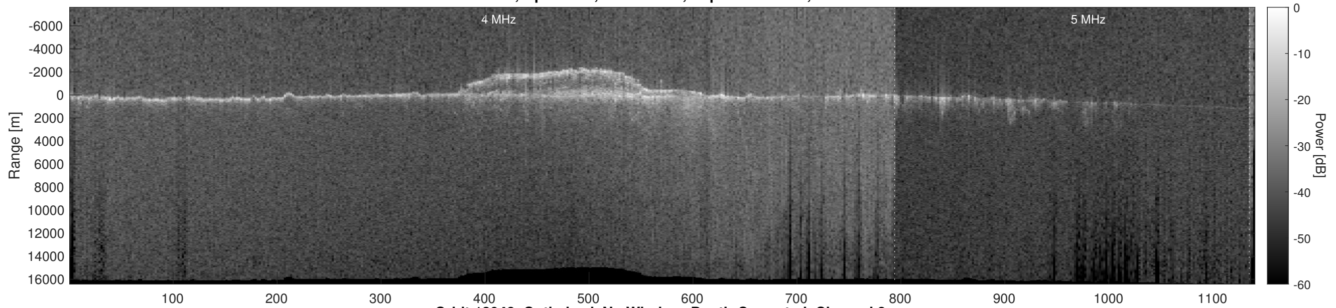
Orbit 13948, Optimized, No Window, Depth-Corrected, Channel 2
