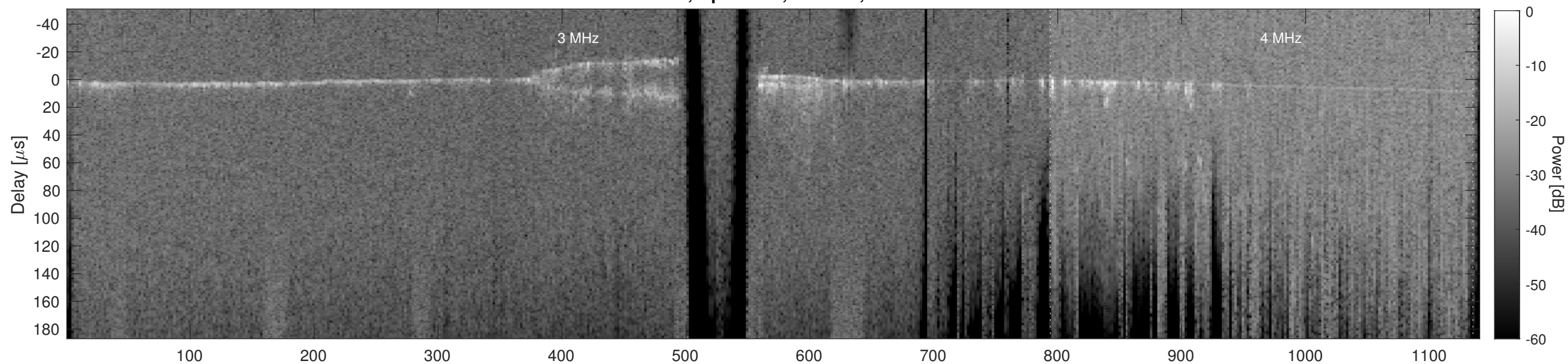
Orbit 13948, Cluttergram
