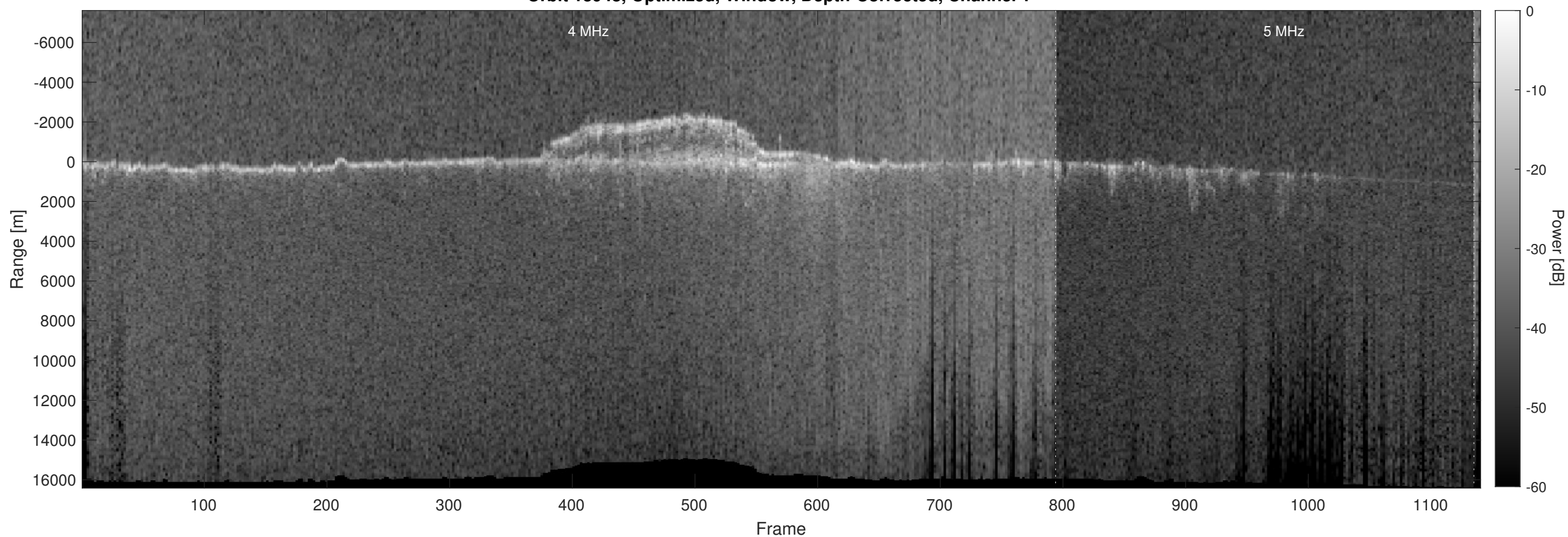
Orbit 13948, Optimized, Window, Depth-Corrected, Channel 2
