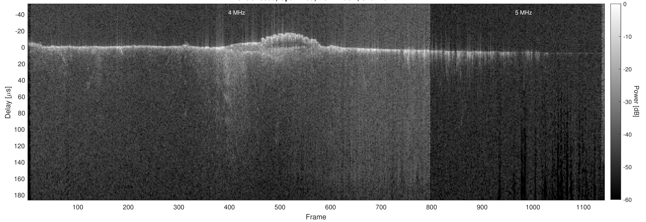
Orbit 13950, Optimized, No Window, Channel 2
