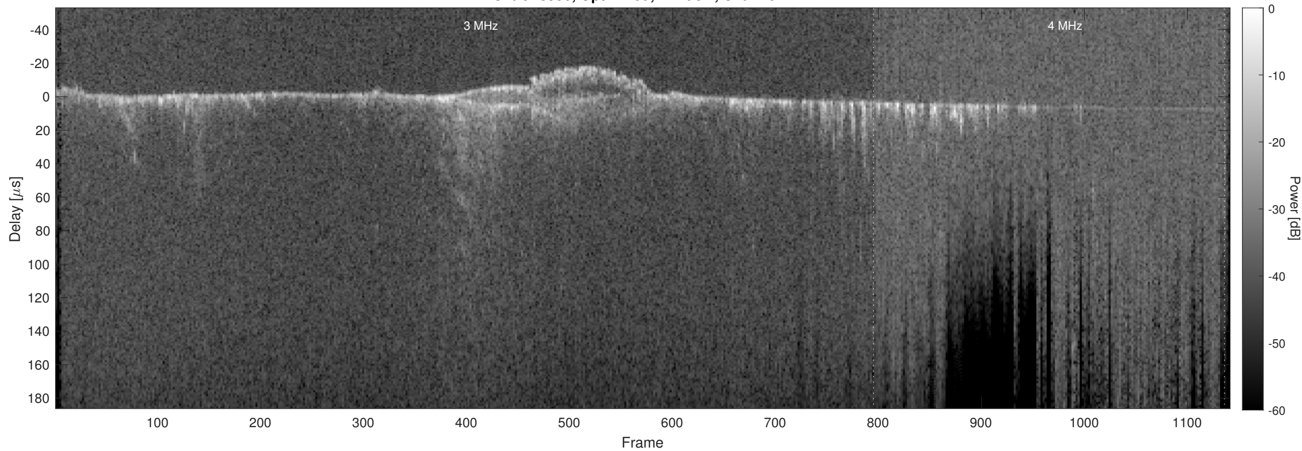
Orbit 13950, Optimized, Window, Channel 2
