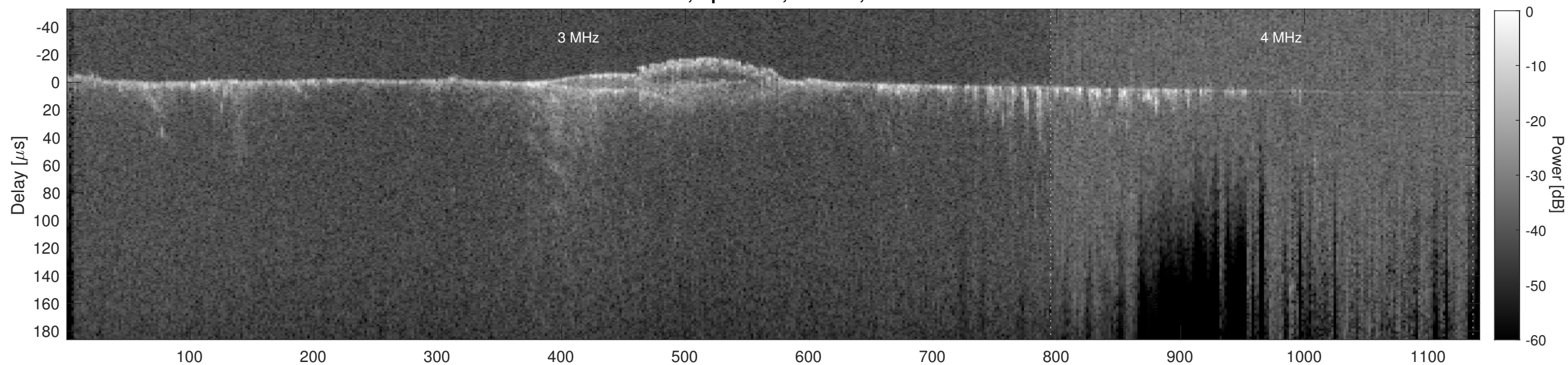
Orbit 13950, Cluttergram
