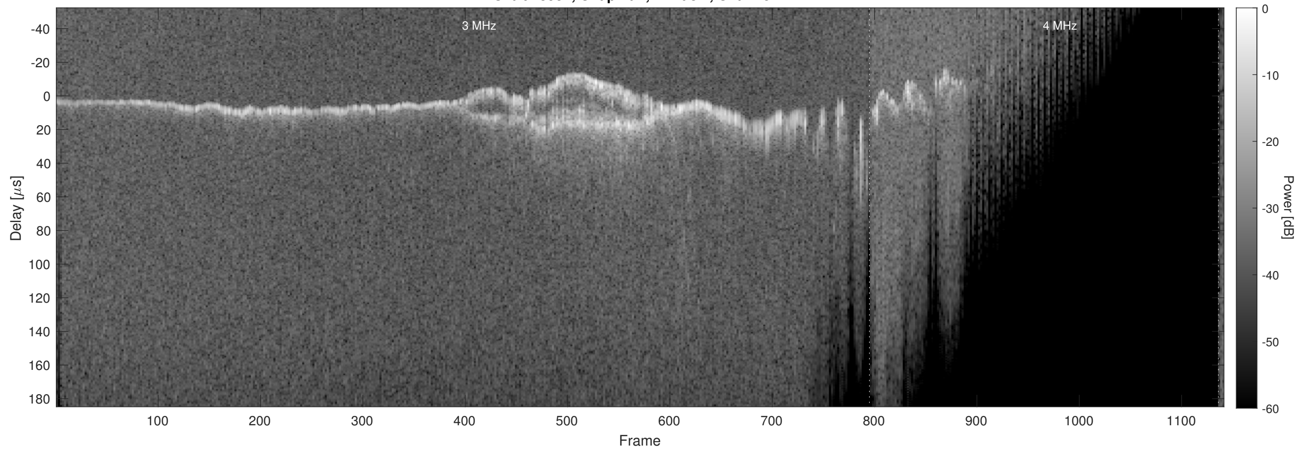
Orbit 13952, Chapman, Window, Channel 2
