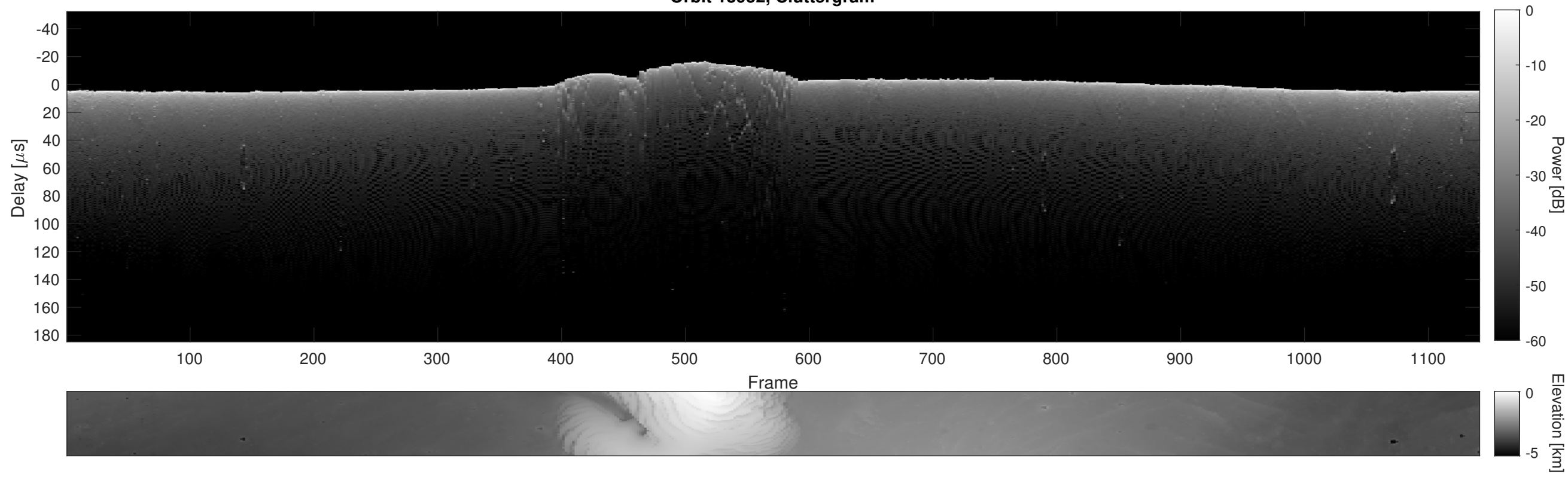
Orbit 13952, Cluttergram
