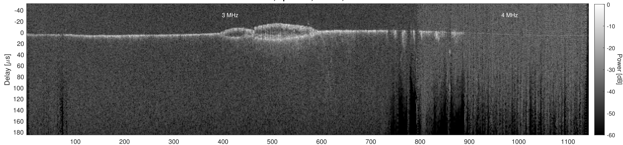
Orbit 13952, Cluttergram
