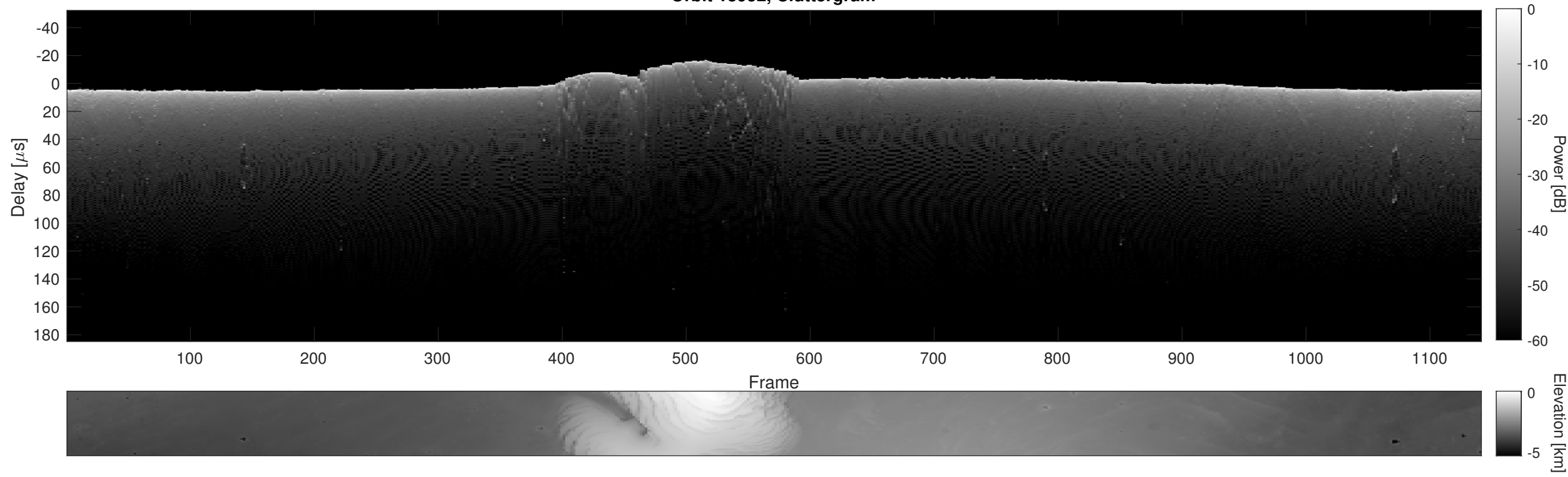
Orbit 13952, Cluttergram
