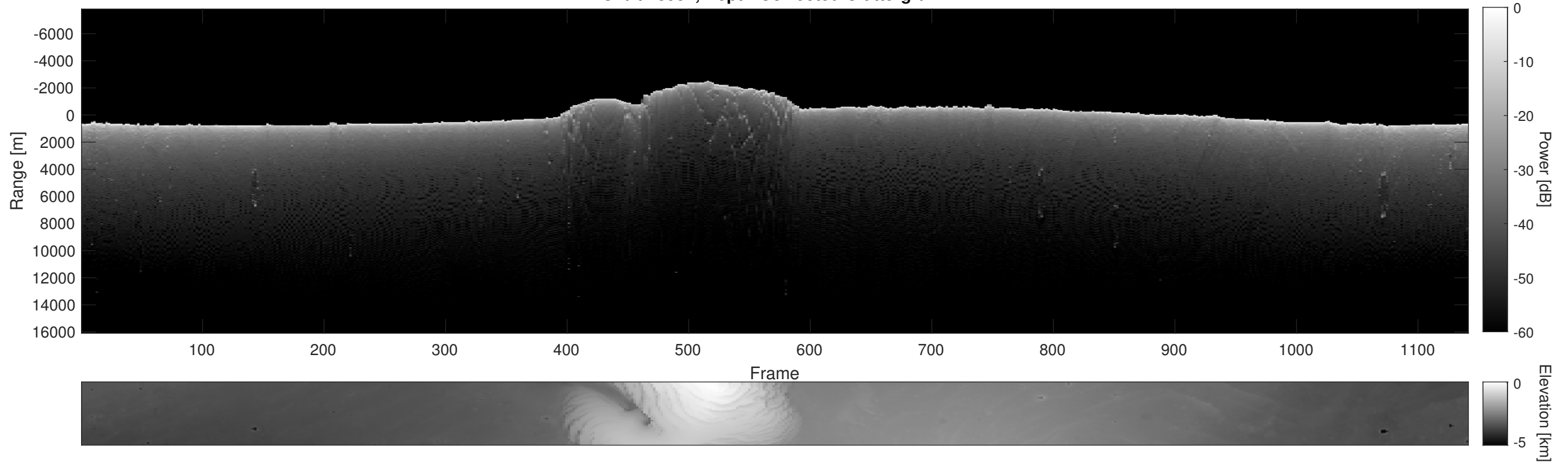
Orbit 13952, Depth-Corrected Cluttergram
