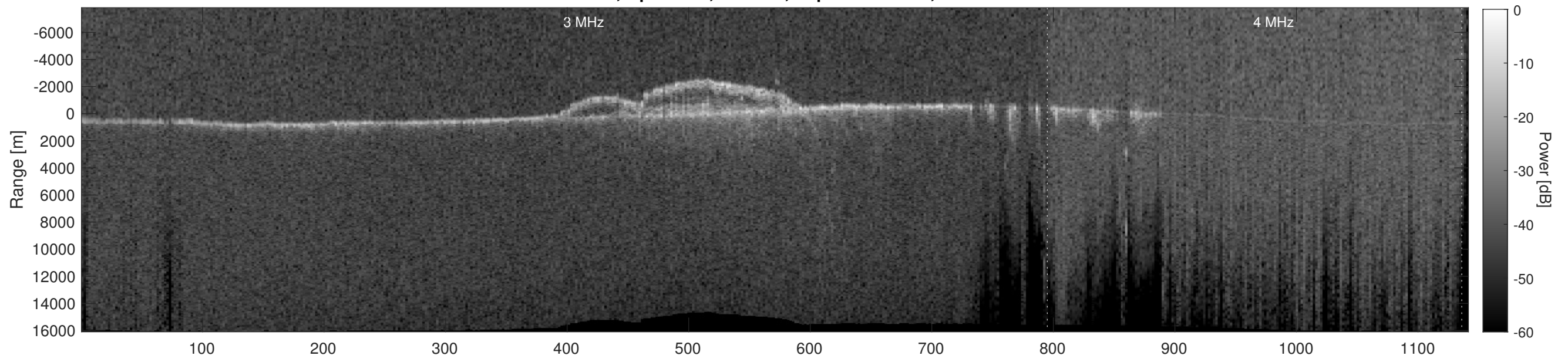
Orbit 13952, Depth-Corrected Cluttergram
