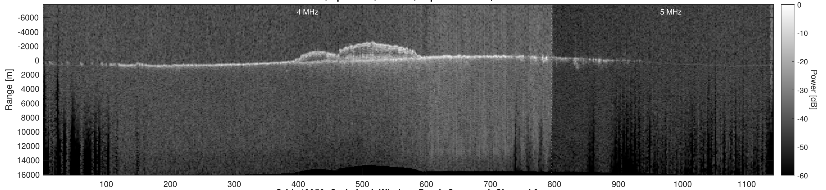
Orbit 13952, Optimized, Window, Depth-Corrected, Channel 2
