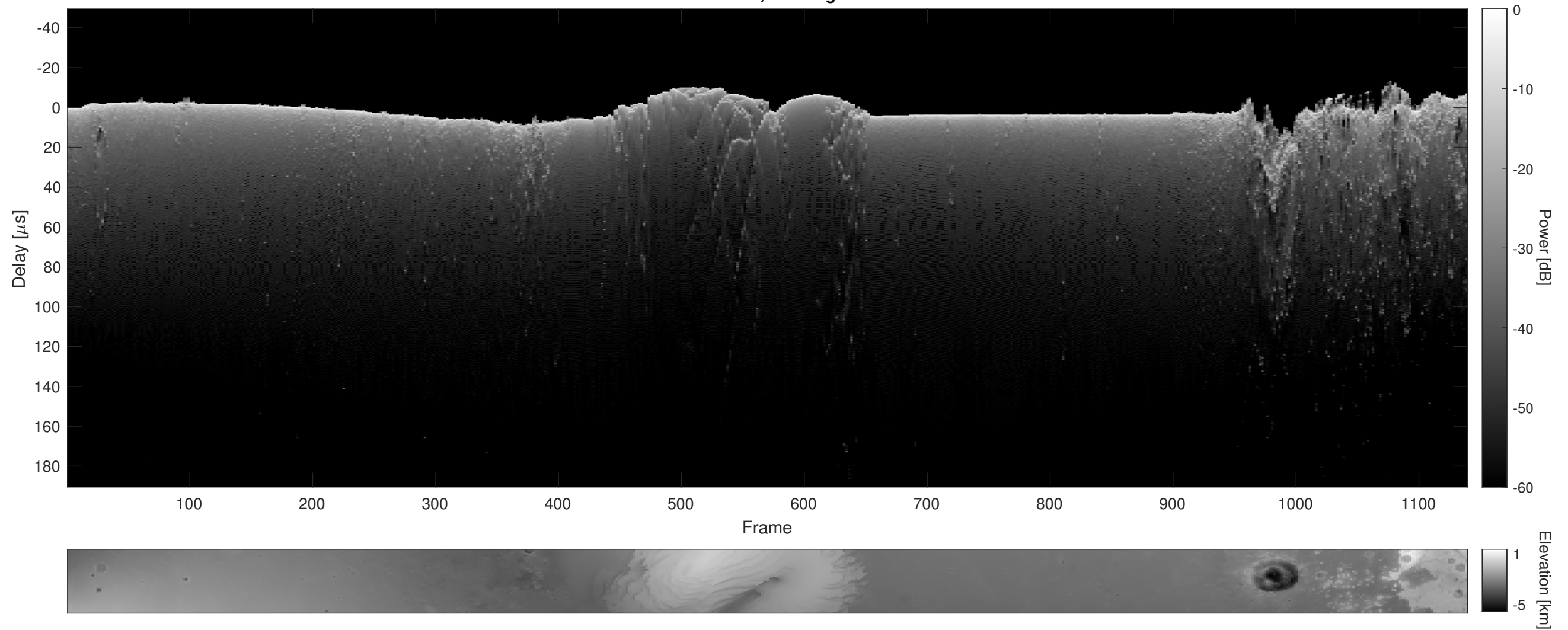
Orbit 13960, Cluttergram
