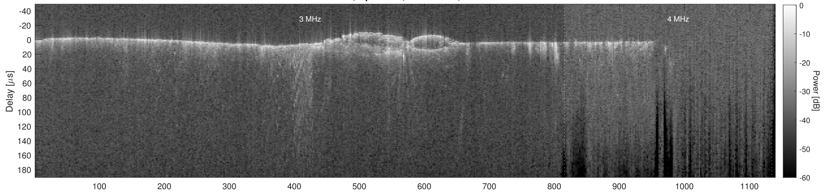
Orbit 13960, Cluttergram
