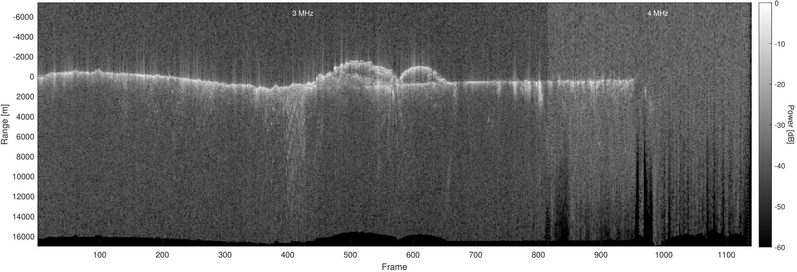
Orbit 13960, Optimized, No Window, Depth-Corrected, Channel 2
