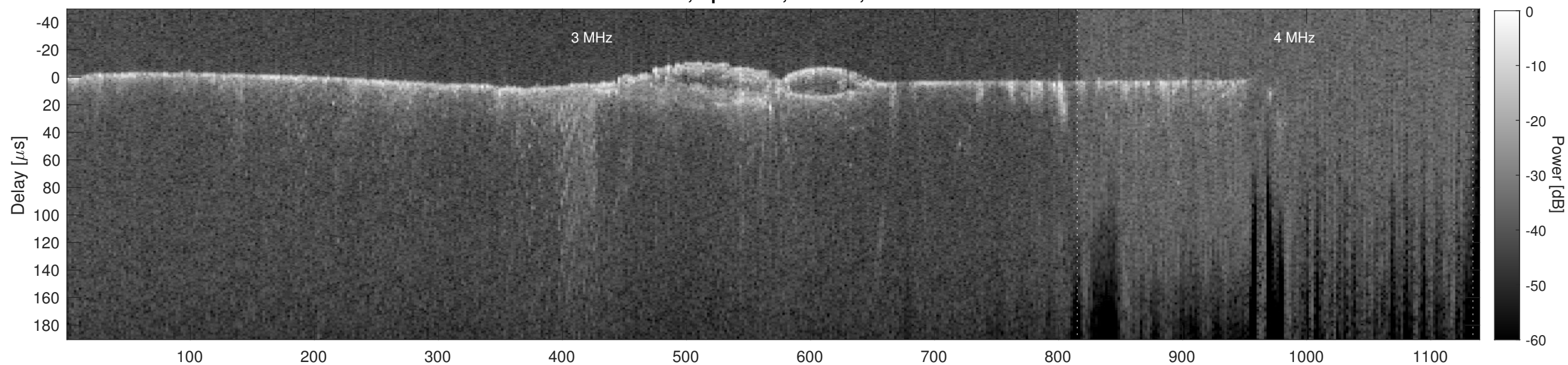
Orbit 13960, Cluttergram
