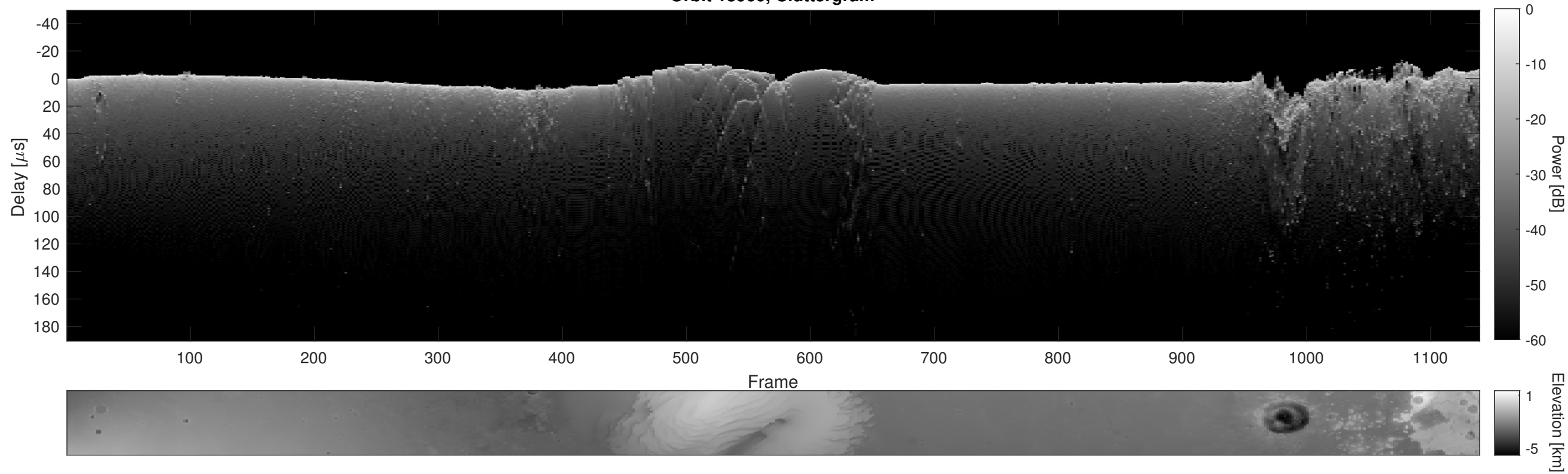
Orbit 13960, Cluttergram
