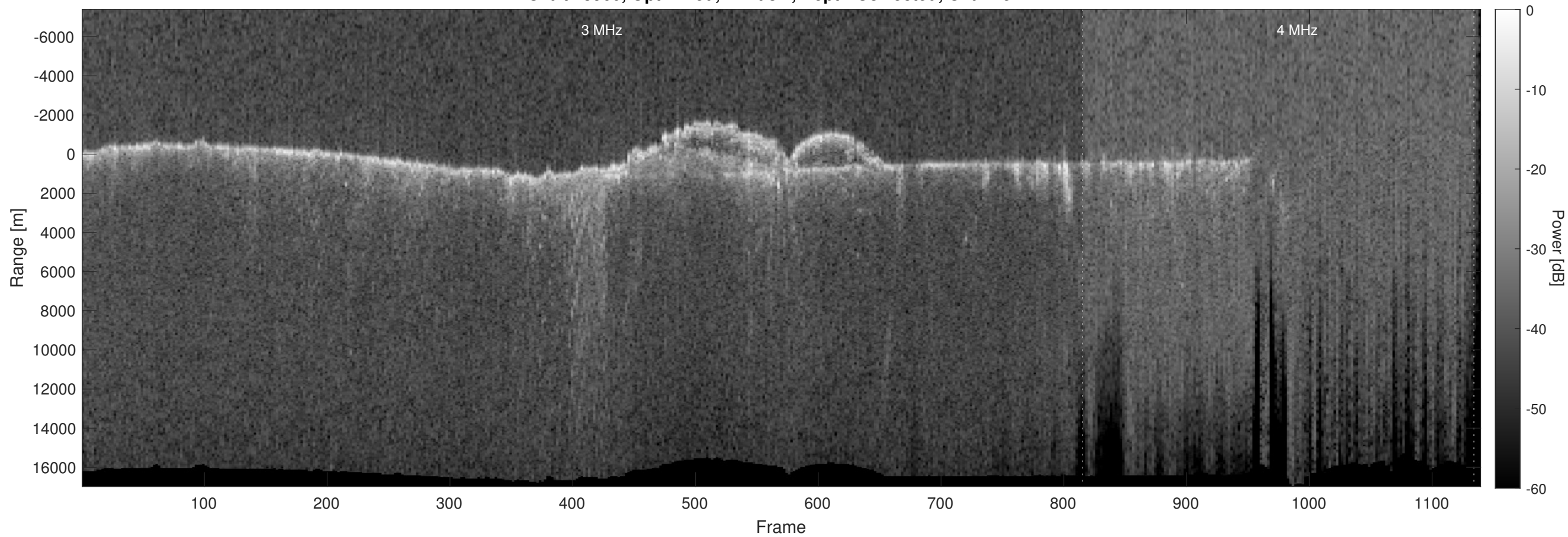
Orbit 13960, Optimized, Window, Depth-Corrected, Channel 2
