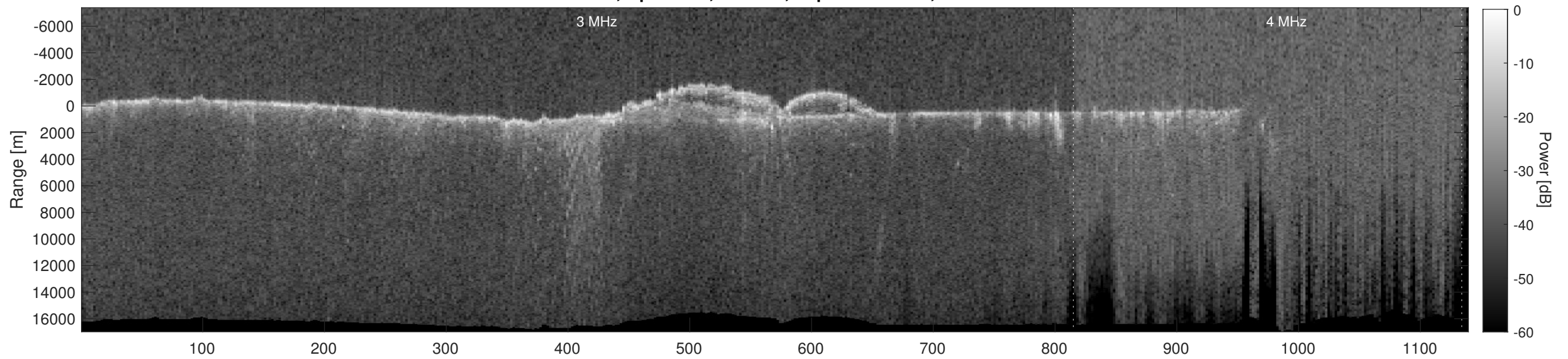
Orbit 13960, Depth-Corrected Cluttergram
