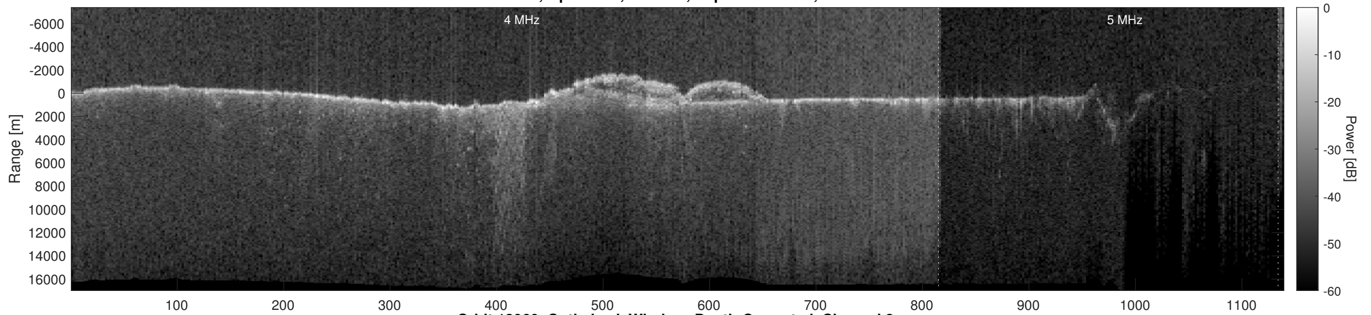
Orbit 13960, Optimized, Window, Depth-Corrected, Channel 2
