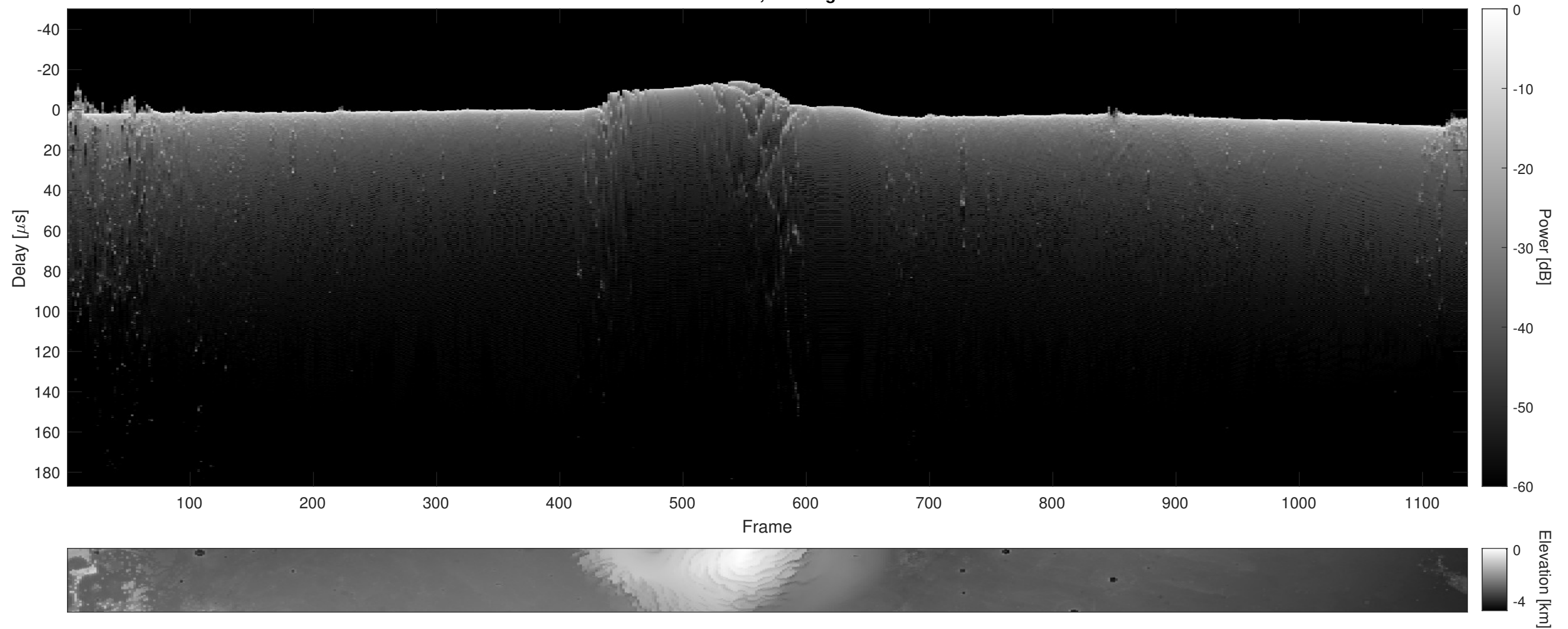
Orbit 13969, Cluttergram
