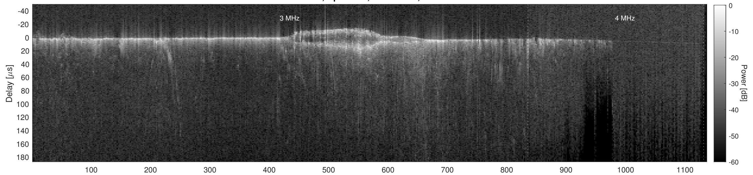
Orbit 13969, Cluttergram
