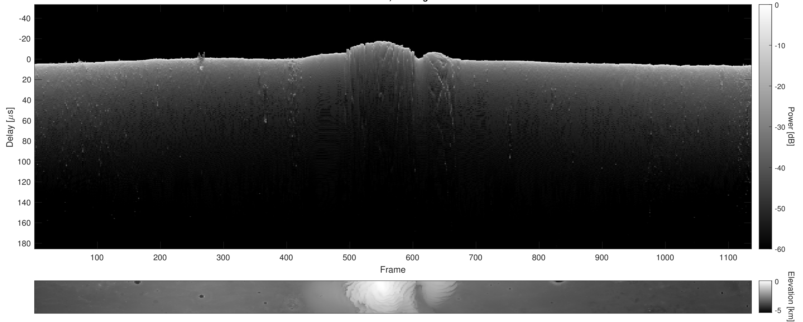
Orbit 13971, Cluttergram
