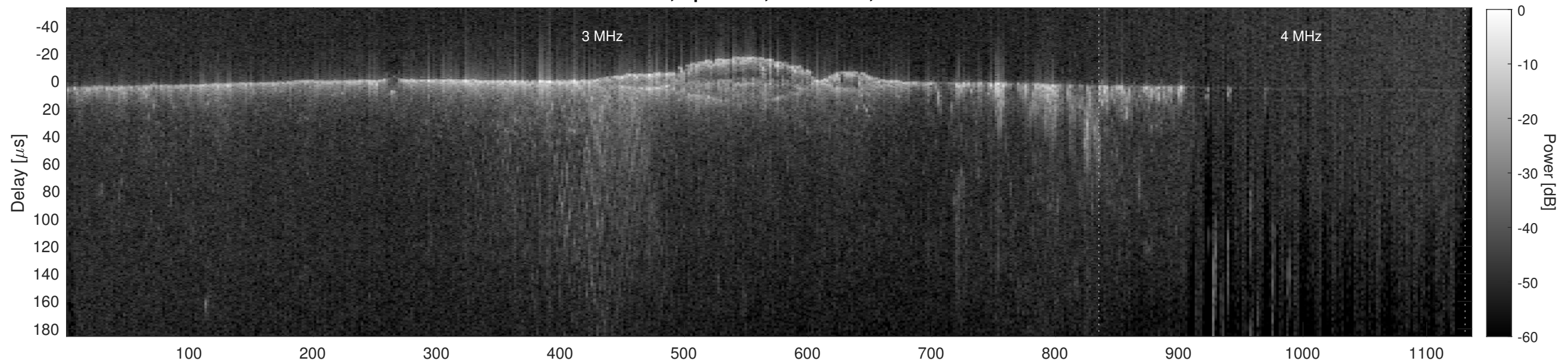
Orbit 13971, Cluttergram
