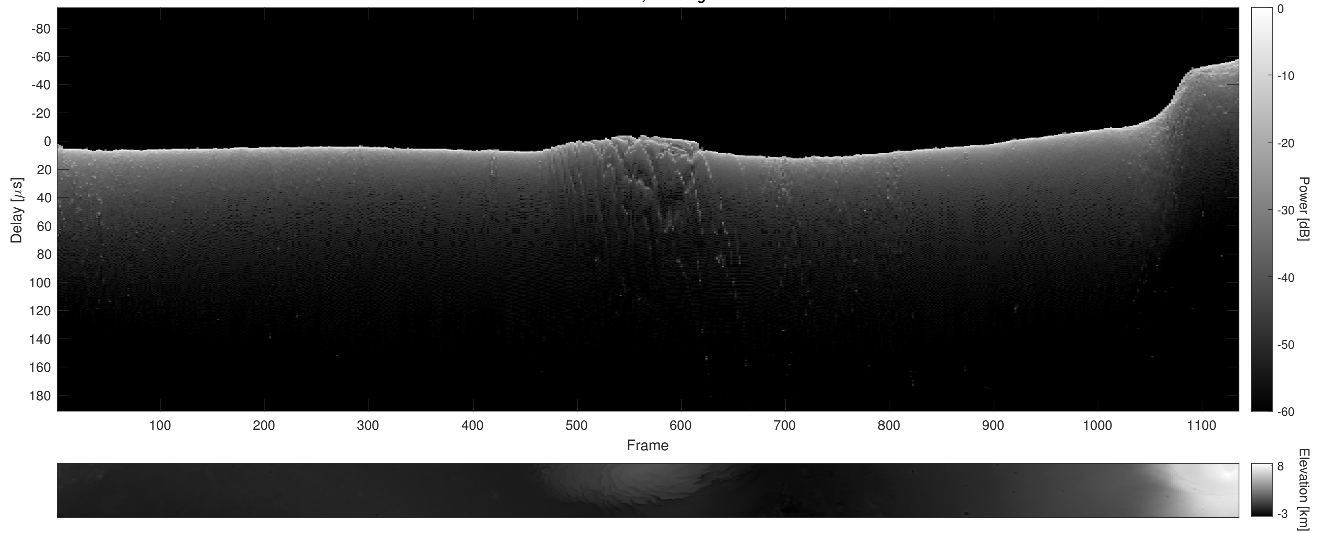
Orbit 13979, Cluttergram
