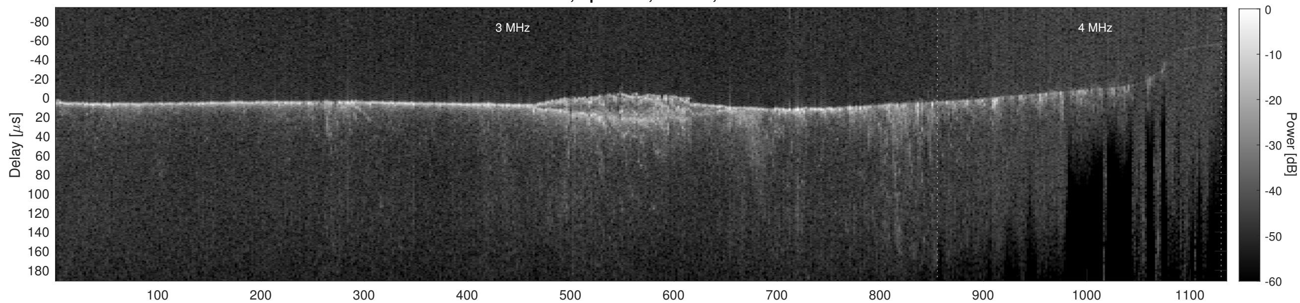
Orbit 13979, Cluttergram
