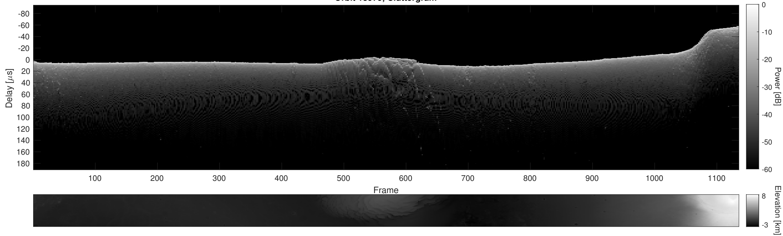
Orbit 13979, Cluttergram
