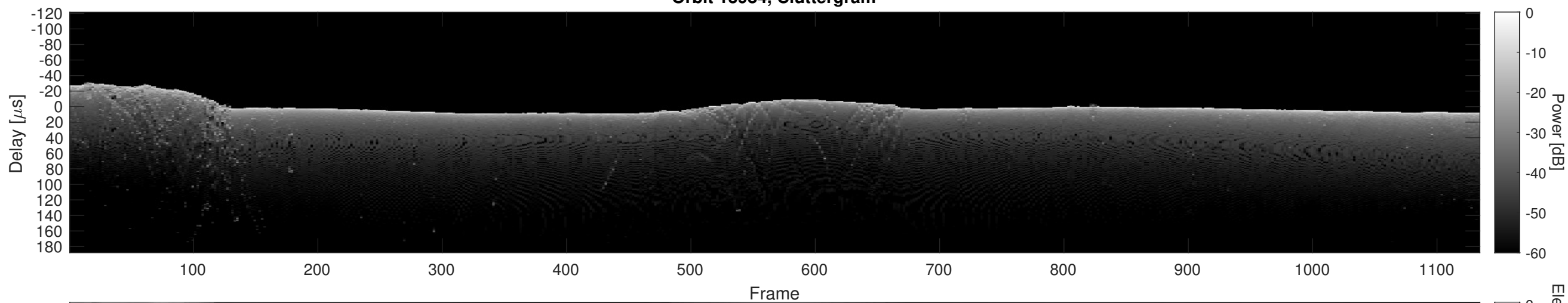
Orbit 13984, Cluttergram
