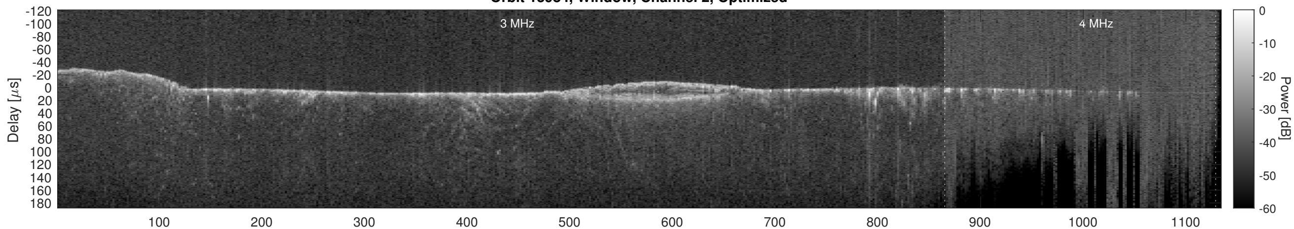
Orbit 13984, Cluttergram
