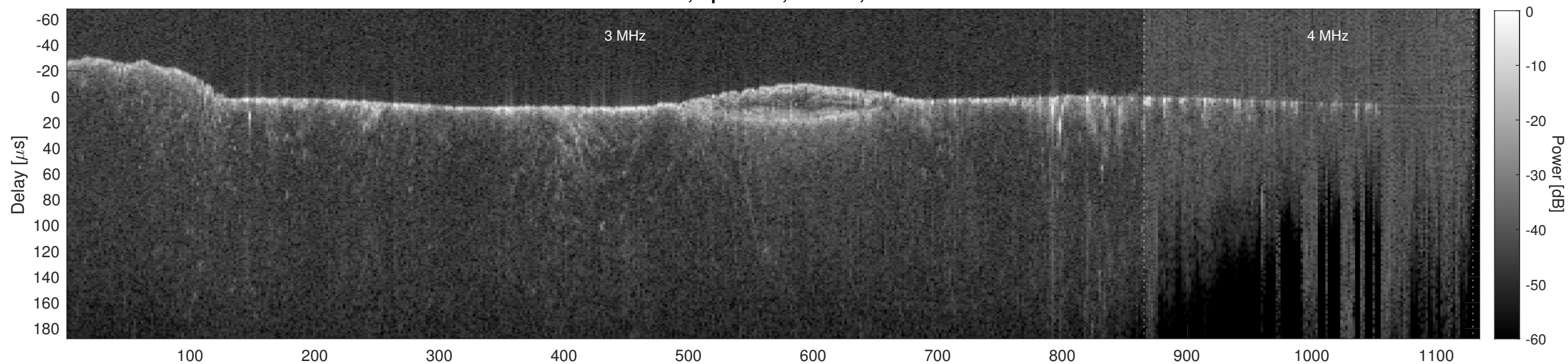
Orbit 13984, Cluttergram
