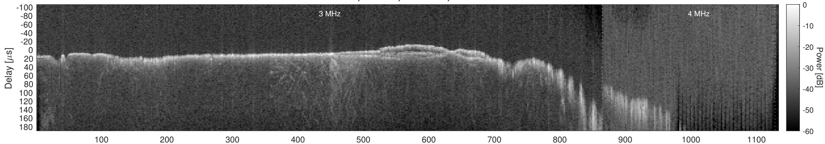
Orbit 13985, Window, Channel 2, Chapman
