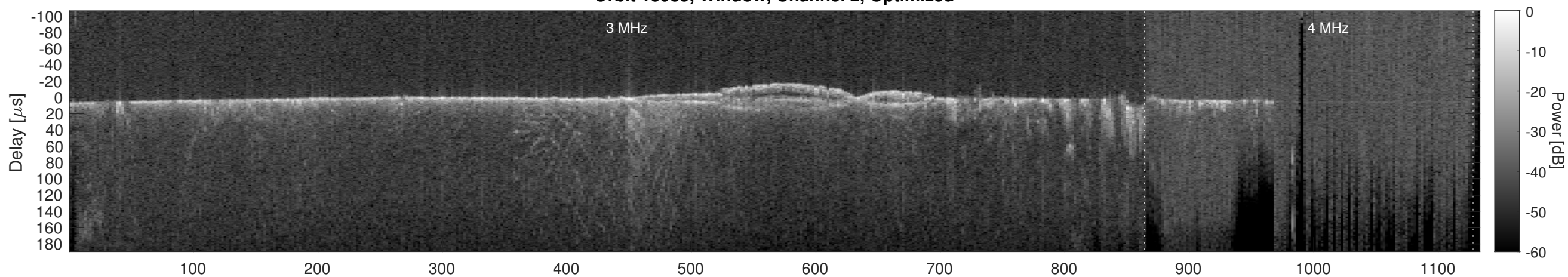
Orbit 13985, Cluttergram
