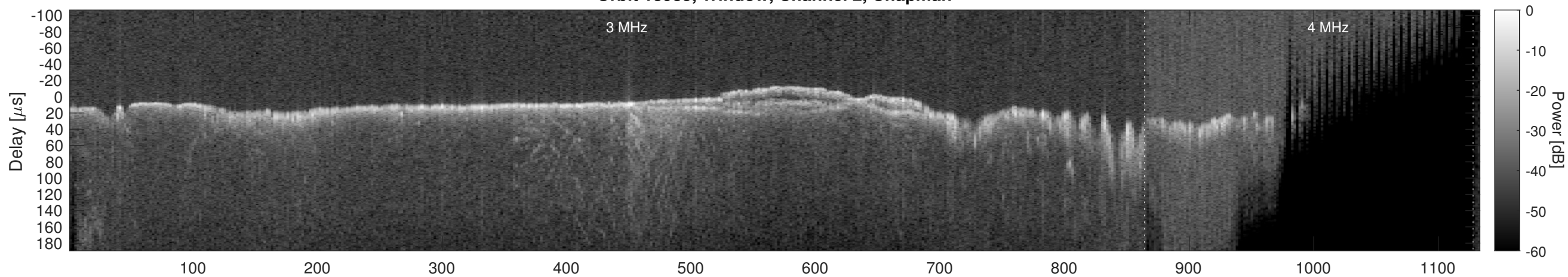
Orbit 13985, Window, Channel 2, Optimized
