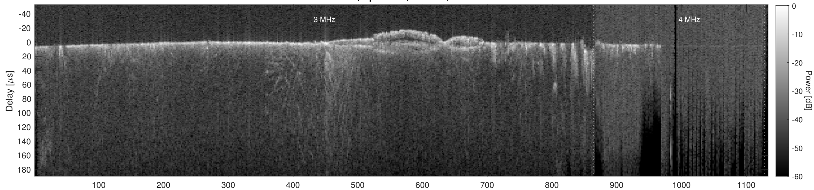
Orbit 13985, Cluttergram
