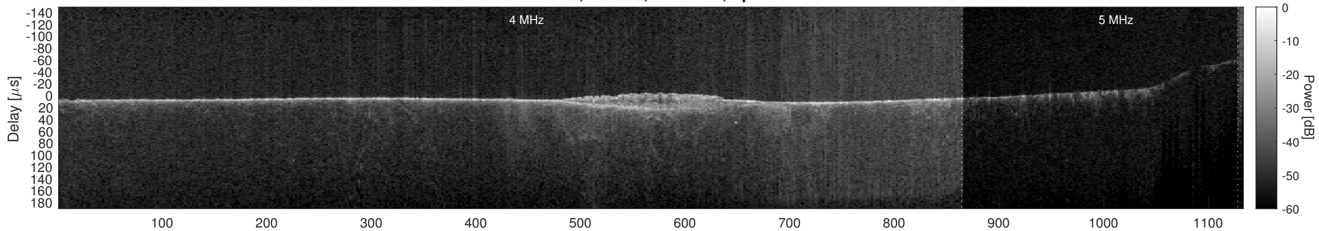
Orbit 13986, Cluttergram
