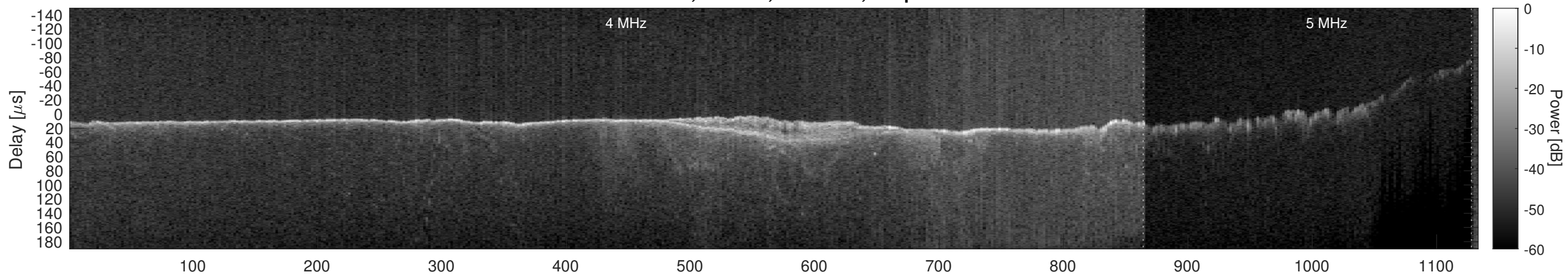
Orbit 13986, Window, Channel 1, Optimized
