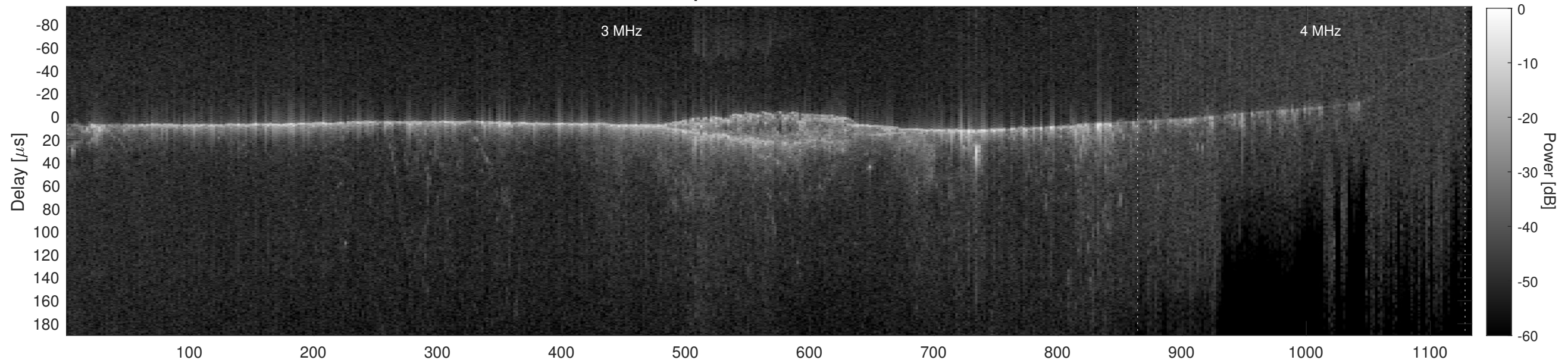
Orbit 13986, Cluttergram
