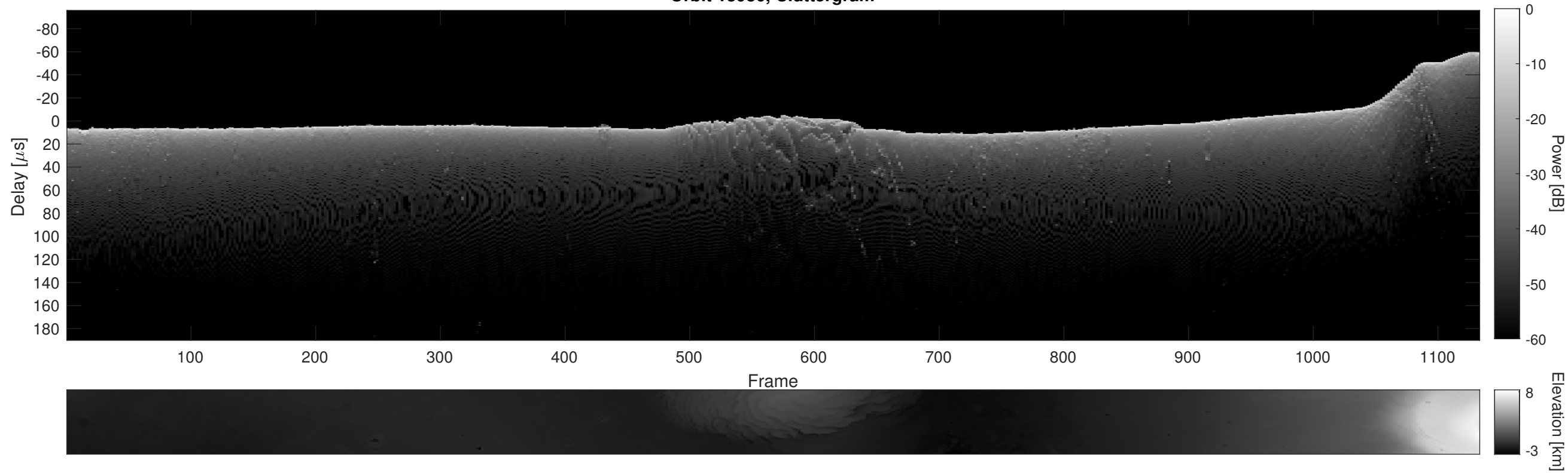
Orbit 13986, Cluttergram
