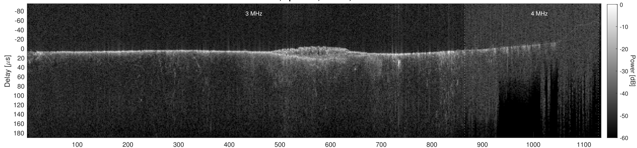
Orbit 13986, Cluttergram
