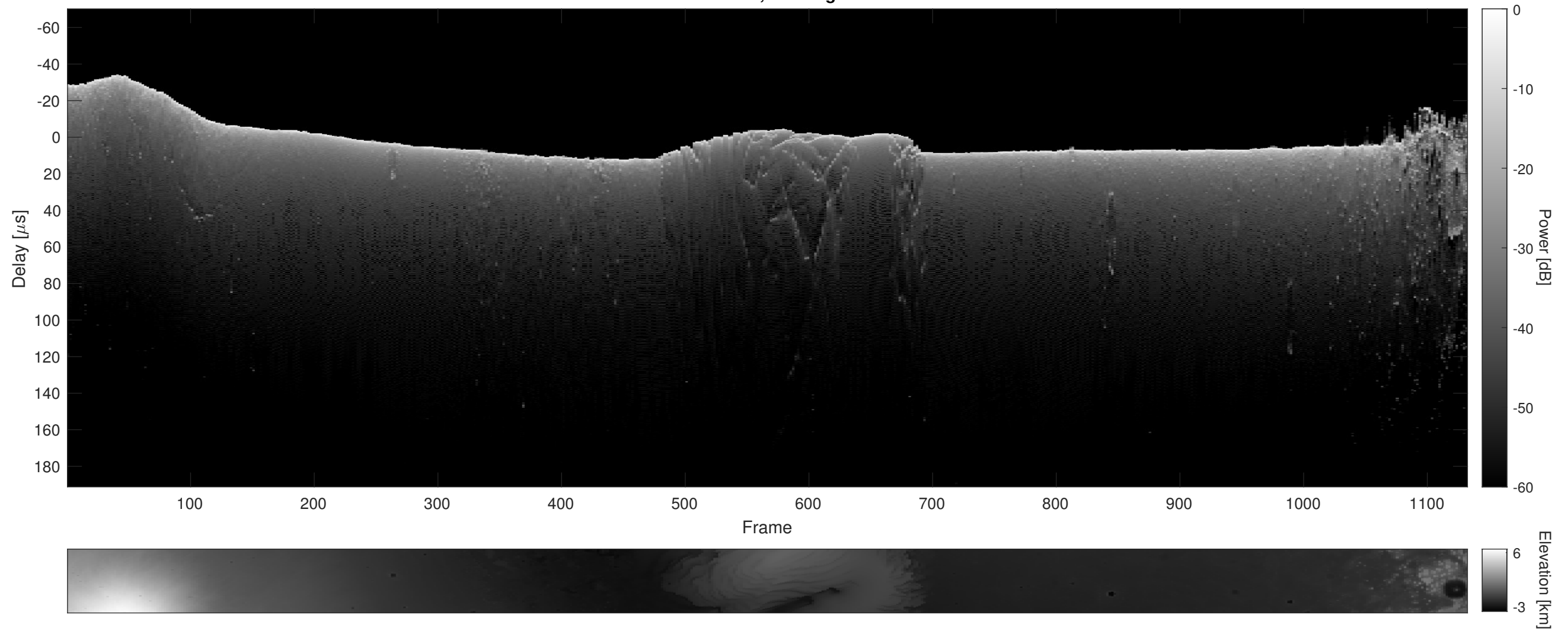
Orbit 13988, Cluttergram
