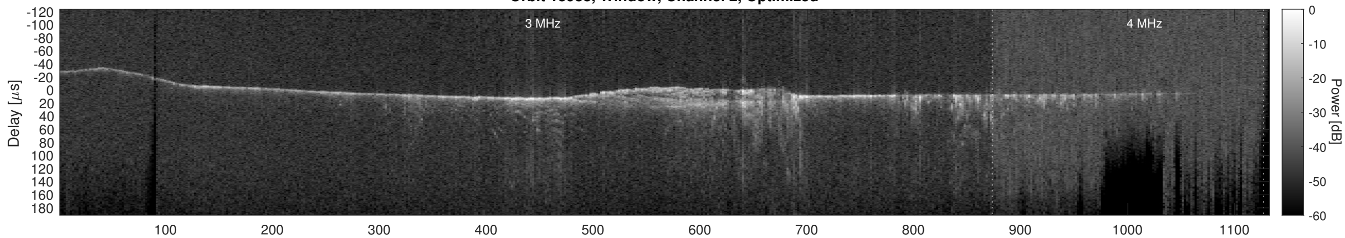
Orbit 13988, Cluttergram
