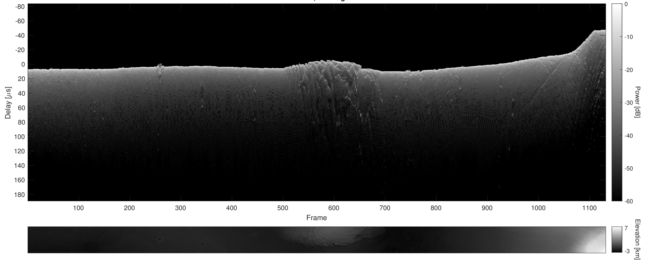
Orbit 13993, Cluttergram
