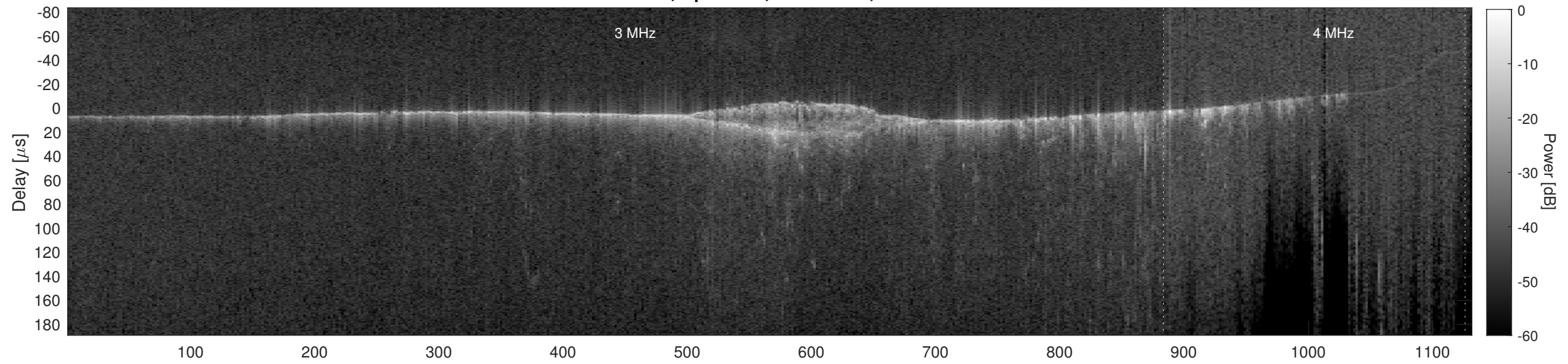
Orbit 13993, Cluttergram
