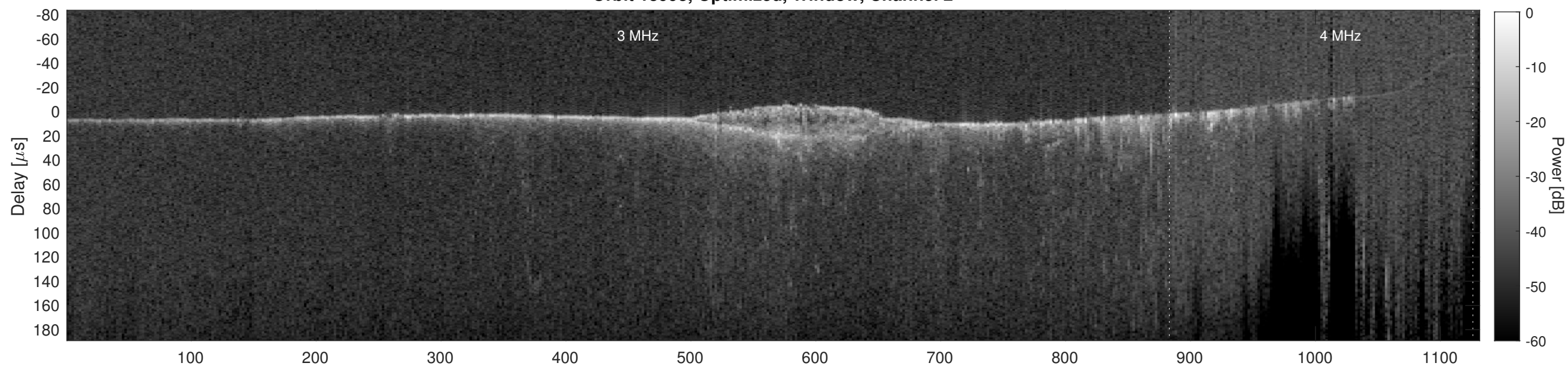
Orbit 13993, Cluttergram
