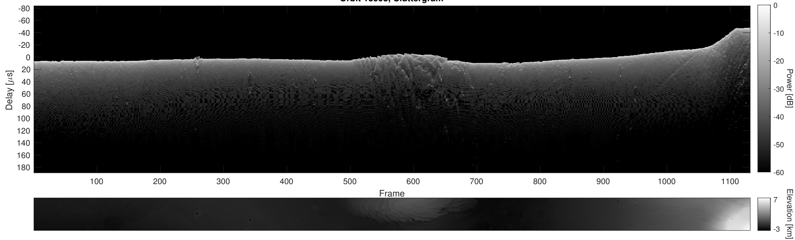
Orbit 13993, Cluttergram
