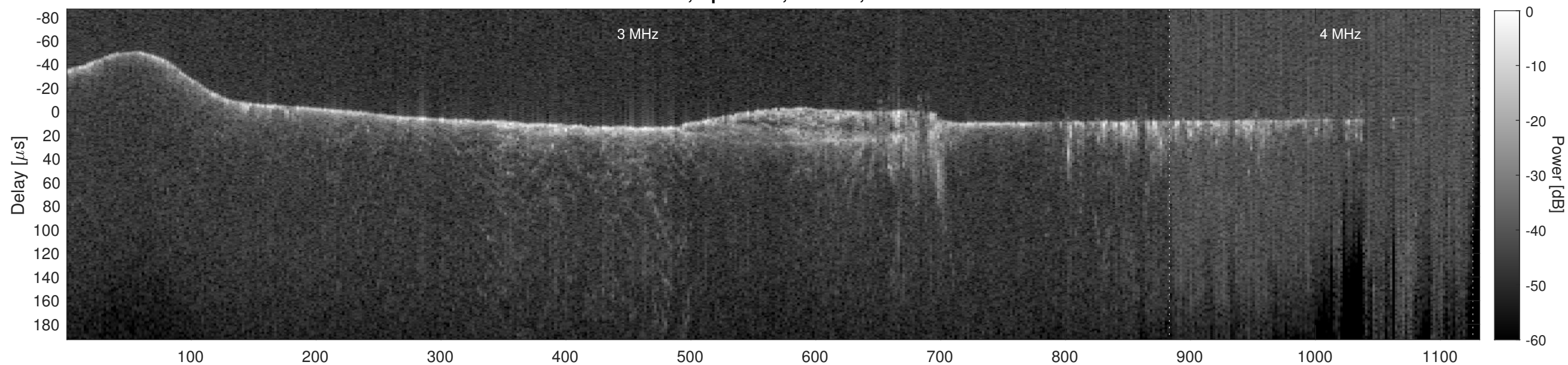
Orbit 13995, Cluttergram
