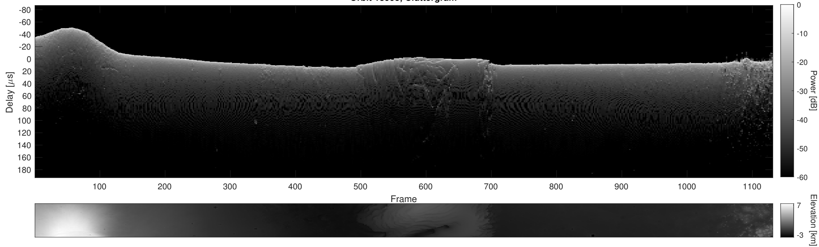
Orbit 13995, Cluttergram
