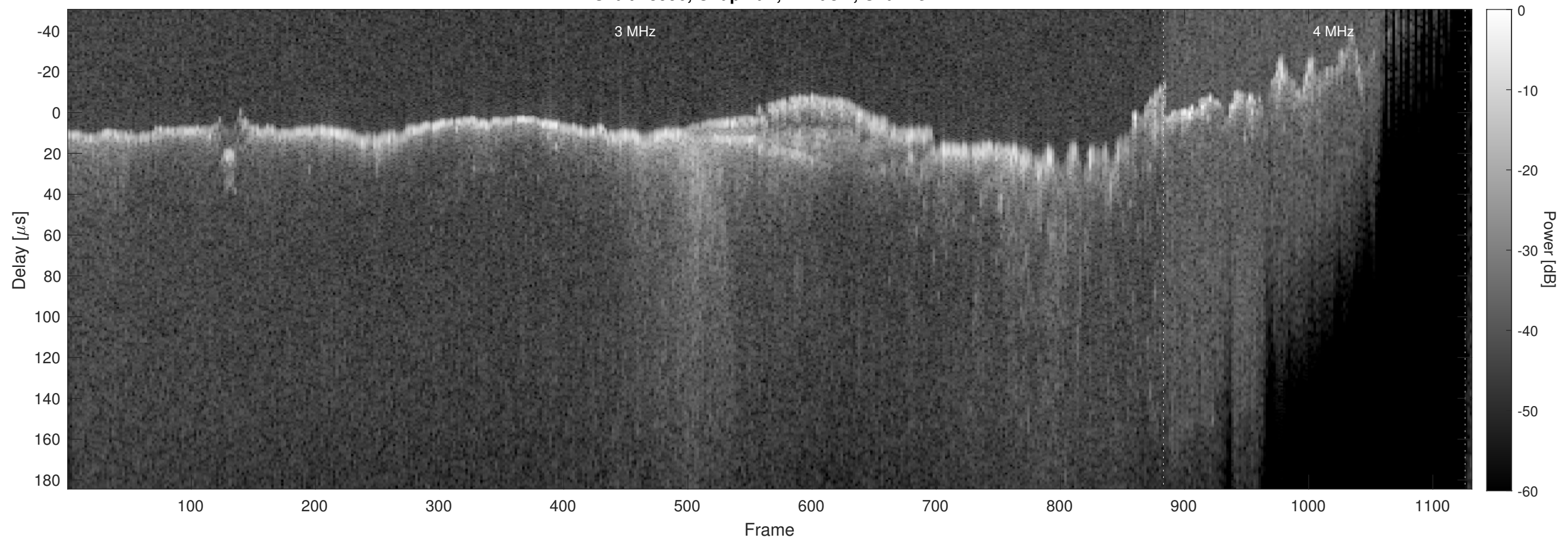
Orbit 13996, Chapman, Window, Channel 2
