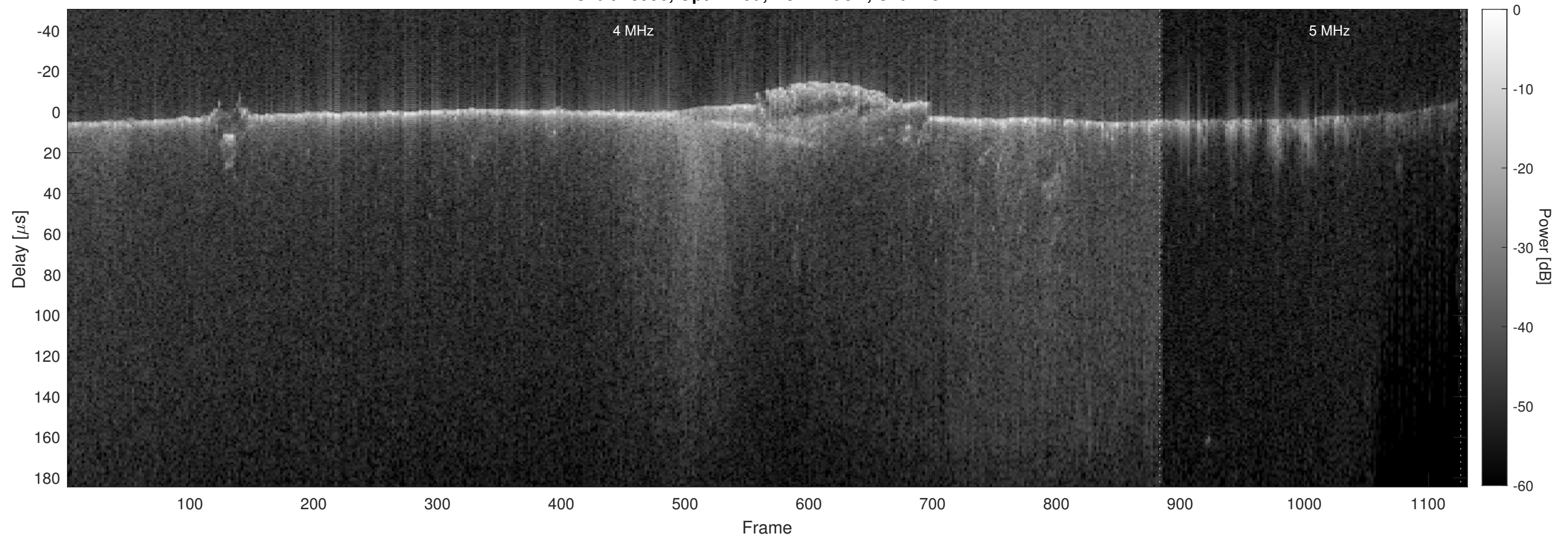
Orbit 13996, Optimized, No Window, Channel 2
