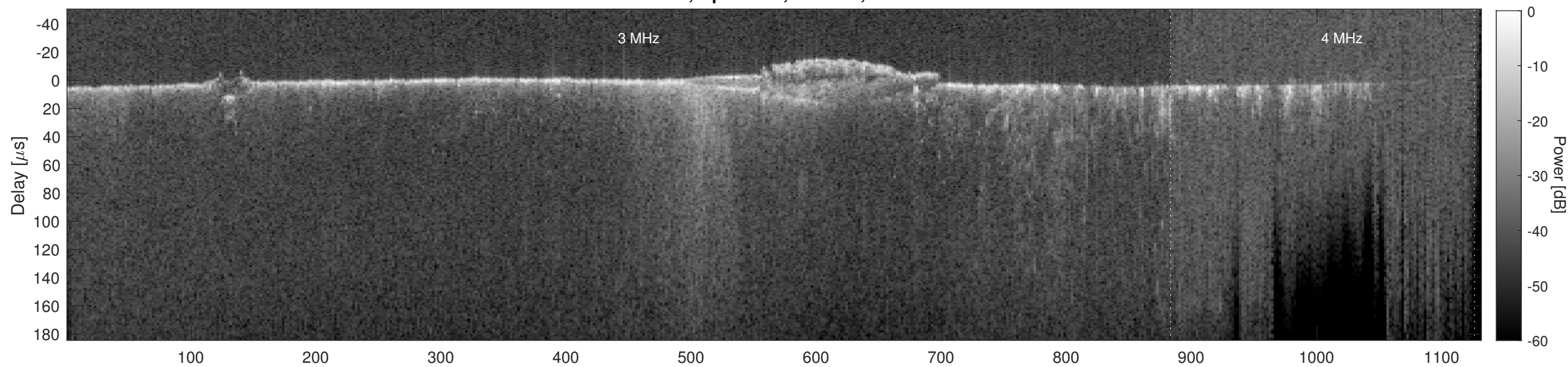
Orbit 13996, Cluttergram
