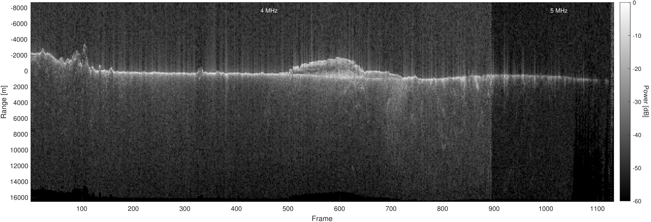
Orbit 13997, Optimized, No Window, Depth-Corrected, Channel 2
