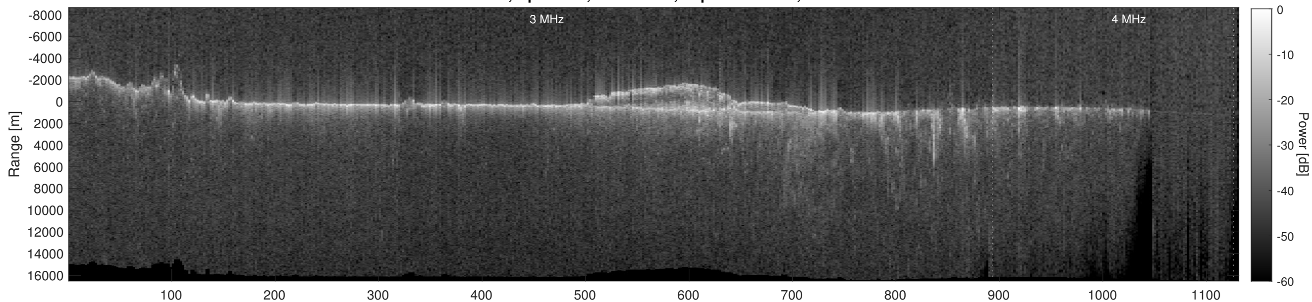
Orbit 13997, Depth-Corrected Cluttergram
