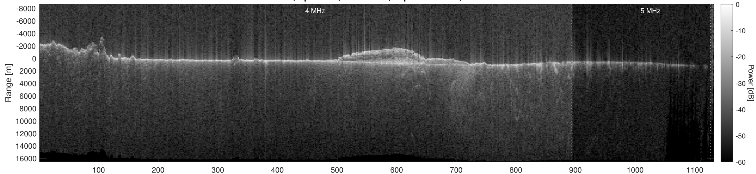
Orbit 13997, Optimized, No Window, Depth-Corrected, Channel 2
