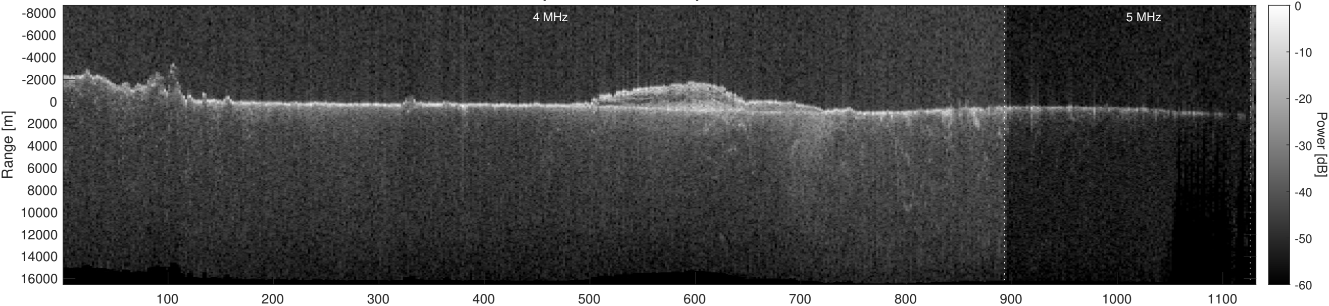
Orbit 13997, Optimized, Window, Depth-Corrected, Channel 2
