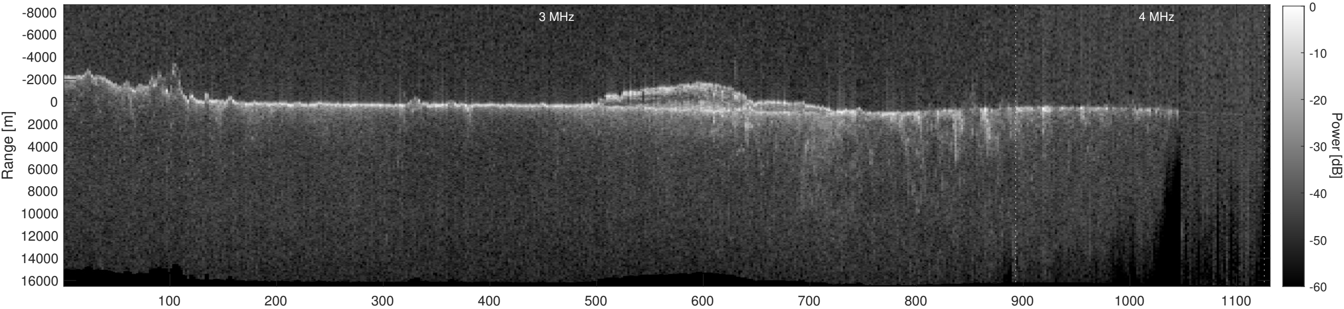
Orbit 13997, Depth-Corrected Cluttergram
