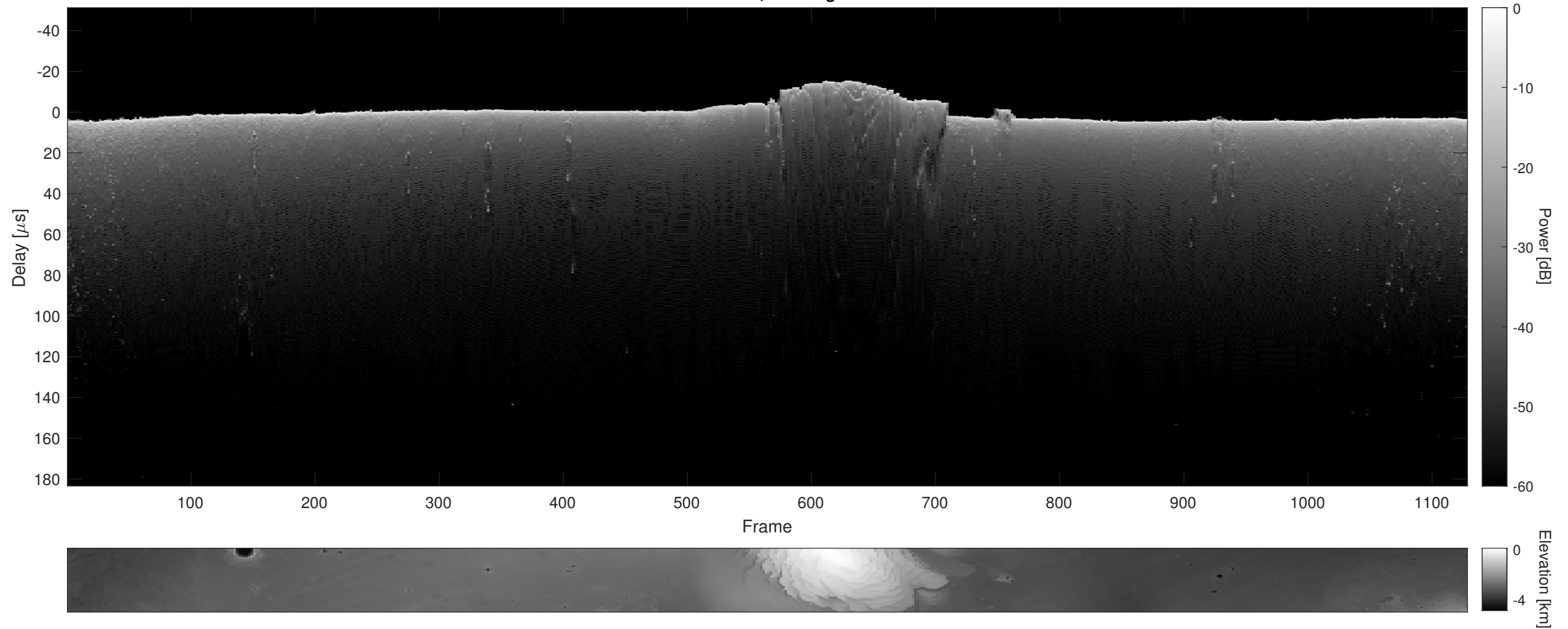
Orbit 14003, Cluttergram
