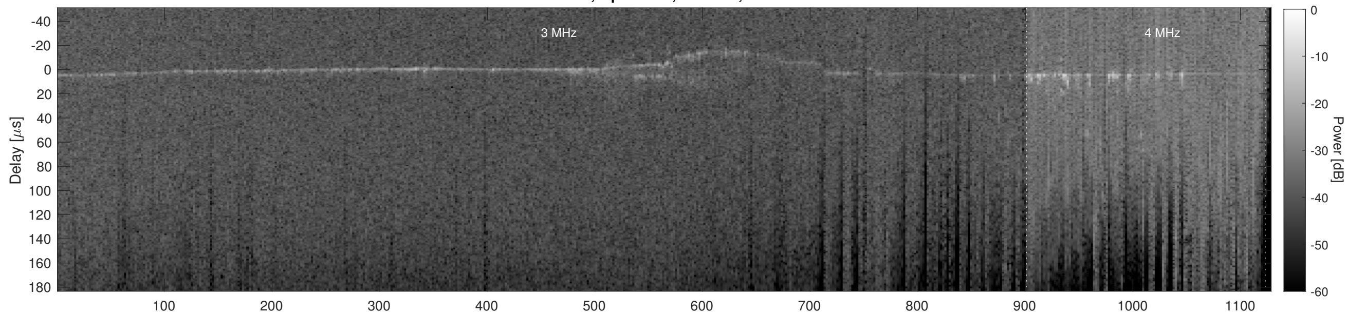
Orbit 14003, Cluttergram
