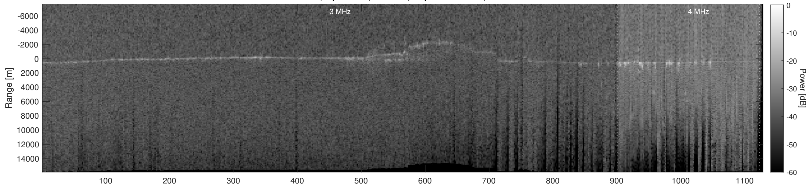
Orbit 14003, Depth-Corrected Cluttergram
