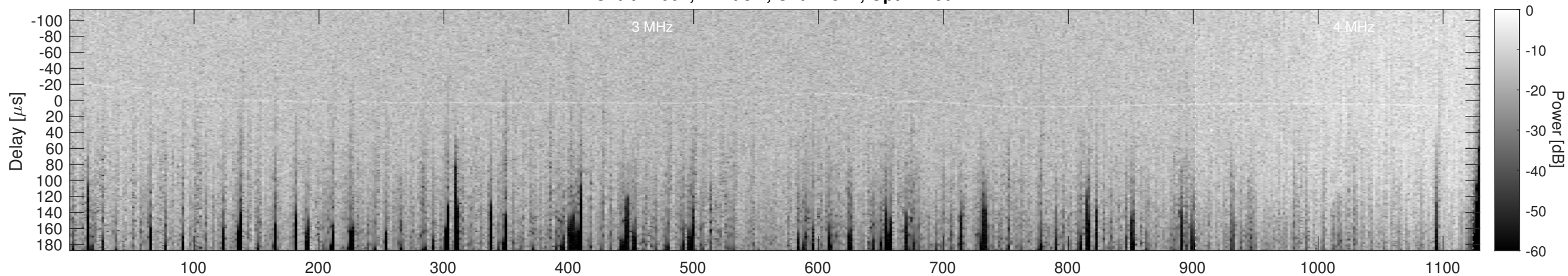
Orbit 14004, Cluttergram
