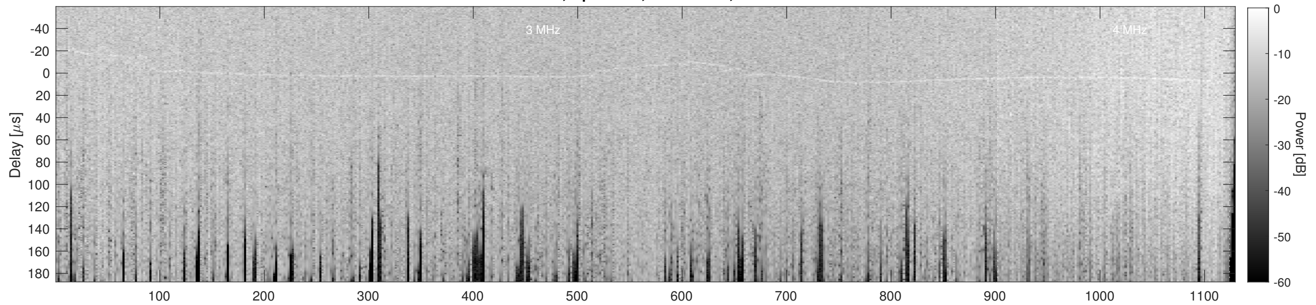
Orbit 14004, Cluttergram
